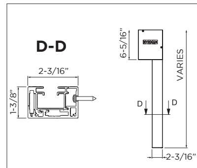
Wall Mounting w/ Direct Screw Connection
