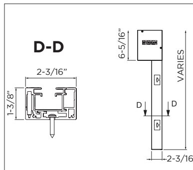
Soffit Mounting
