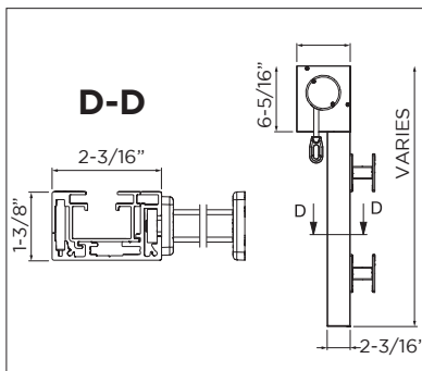
Mounting w/ Fastening Brackets
